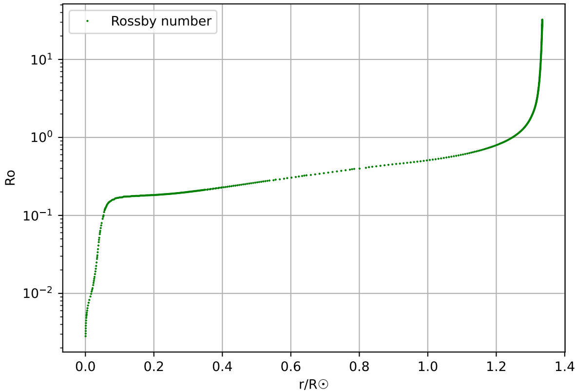
Rossby number, profile 9
